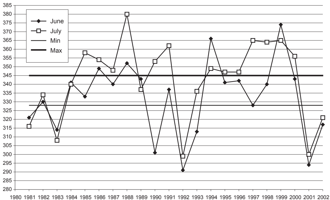
Fig. 2. Water level dynamics on 1 June and 1 July from 1981 through 2002 at monitoring plot I. The minimum and maximum curves indicate the lower and upper limits of water level fluctuations within which conditions for breeding of Aquatic Warbler remain favorable. 345 m above sea corresponds to 12 cm above soil, while 328 m above sea corresponds to 5 cm below soil.
