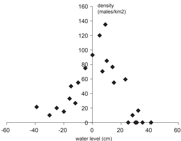
Fig. 1 Change of Aquatic Warbler male density at Sporovskii mire depending on the water level (cm). 0 — ground level, +10 — water level above soil, -10 — water level below soil).
